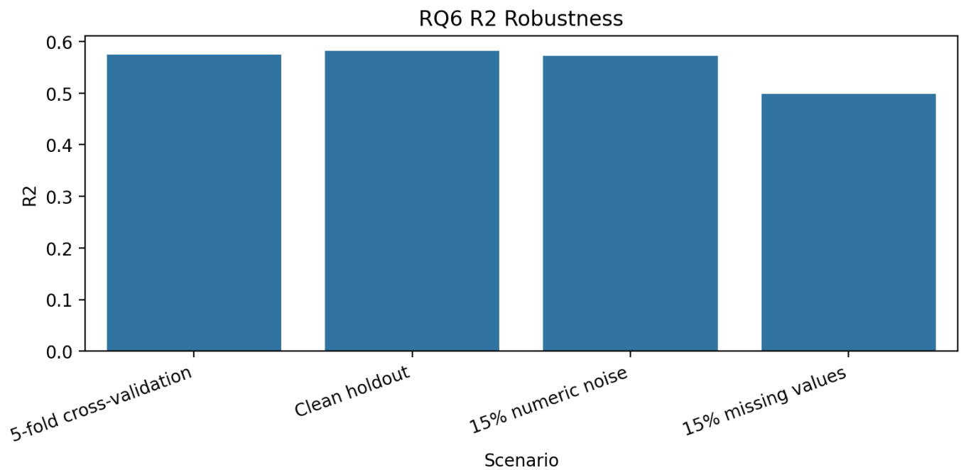
Fig. 7. RQ6: Robustness comparison across clean holdout, cross-validation, noisy input, and missing-value scenarios. Missing data causes the largest performance decrease.
